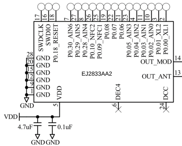
Internal LDO setup
